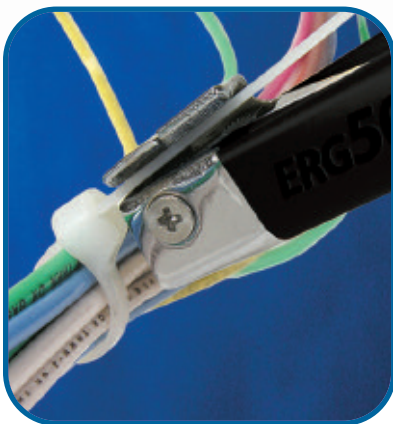
Tightens cable tie and cuts flush in one step
